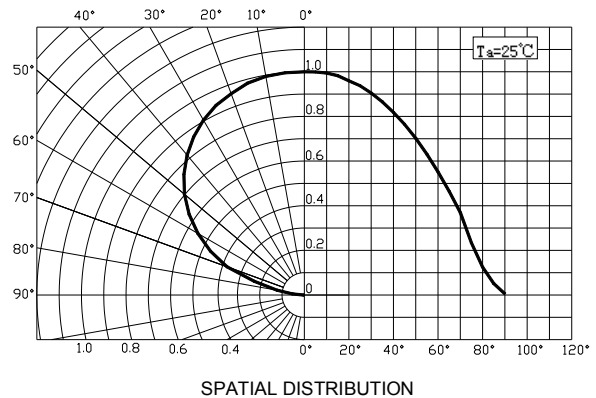
Radiation diagram
